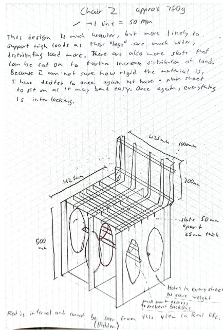
(b) Design 2
