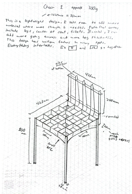
(a) Design 1
